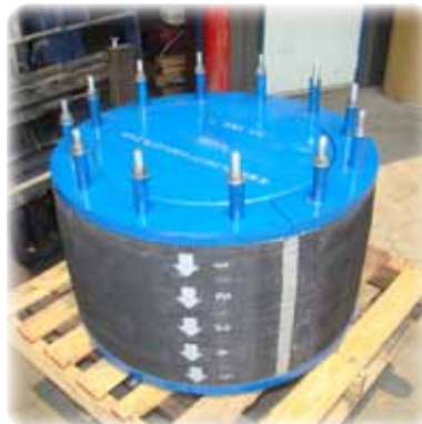
30" High Pressure Mechanical plug. Designed to fit through a 24" manhole.
